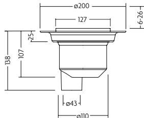
Quad Gravity Drain Slot - Vertical Outlet
