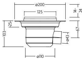
Quad Gravity Drain Tiled Insert 14mm - Horizontal Outlet
