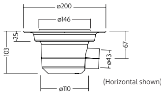
Vinyl Floor Gully - Horizontal Outlet
