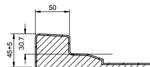
Tray Profile
