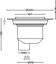
Tiled Floor Gully - Vertical Outlet
