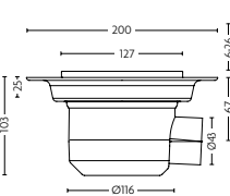
Tiled Floor Gully - Horizontal Outlet
