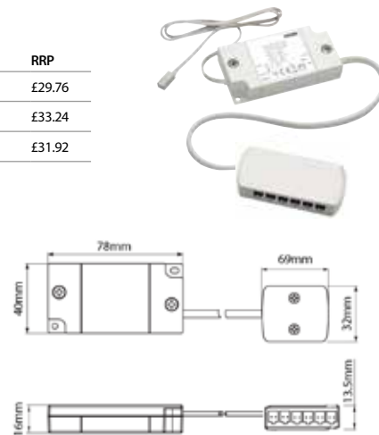
Single colour LED - 12 ports
