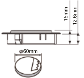
Cut-out size: Ø60mm
