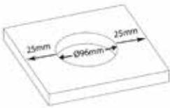
Cut-out Ø96mm
