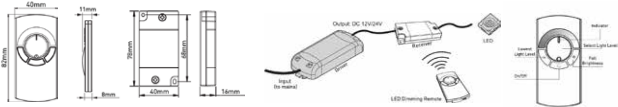
LED Dimming Remote Control
