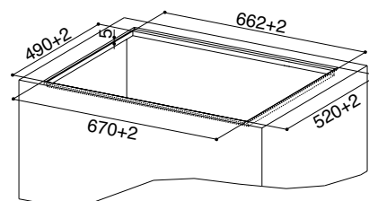
HOO-B + 2 FABER INDUCTION HOBS FCH32 FLUSH FIT INSTALLATION
