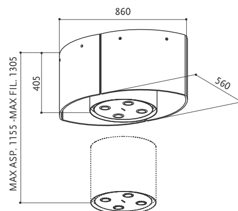
Nest, ducted version
