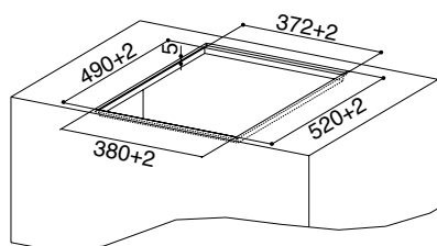
HOO-B GLASS + 1 FABER INDUCTION HOB FCH32 FLUSH FIT INSTALLATION
