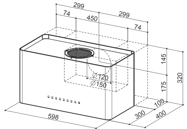
Air outlet adjustable on the rear side
