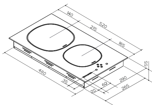
FCH32 - to combine with Hoo-B
