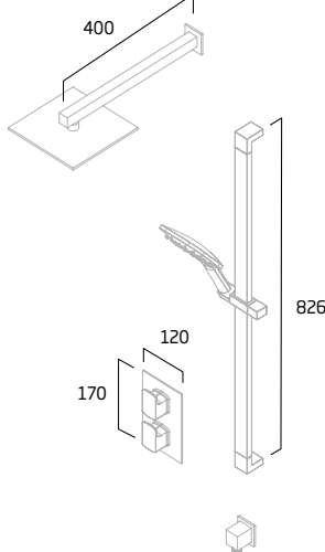
Spirit & Ergo Dual Function Shower System
