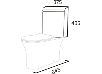
Standard WC Cistern (Fits Fully Enclosed and Open Back WC)
