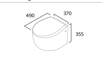
Wall Hung WC
