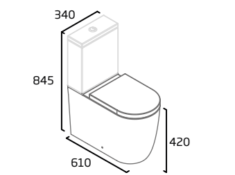
Fully Enclosed Close Coupled WC
