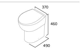
Comfort Height Back To Wall WC
