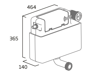
Concealed Dual Flush Cistern (Side Entry Inlet)
