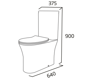
Comfort Height Fully Enclosed Close Coupled WC
