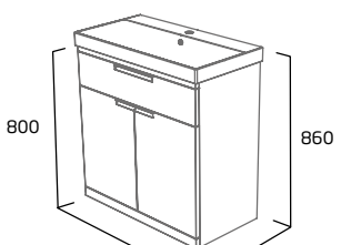
800mm Freestanding Wash Unit
