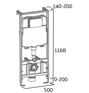
1.17m Wall Hung WC Frame
