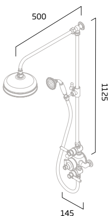
Halcyon Dual Function Shower System
