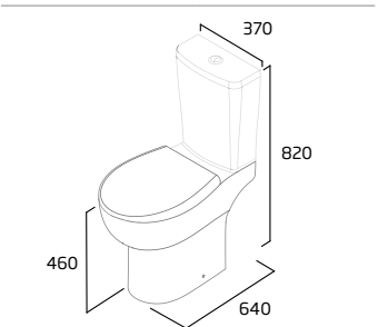
Comfort Height Close Coupled WC
