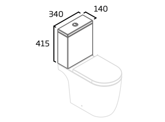
Standard WC Cistern
