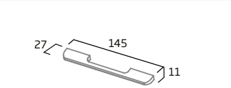
98mm Pull Handle
