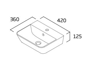
420mm Basin
