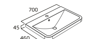
700mm Basin
