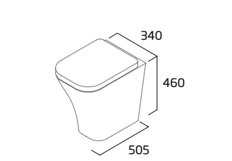
Comfort Height Back To Wall WC
