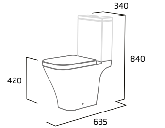
Standard Height Close Coupled WC
