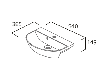
Slim Depth Semi-Countertop Basin
