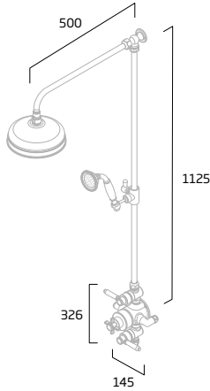
Ashton & Regatta Dual Function Shower System
