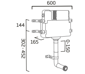
In-Wall Cistern
