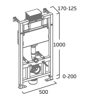
1.0m Wall Hung WC Frame
