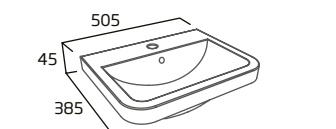
500mm Basin
