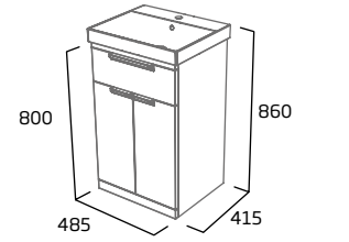
500mm Freestanding Wash Unit
