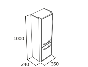
350mm Wall Column
