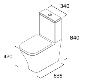
Fully Enclosed Close Coupled WC
