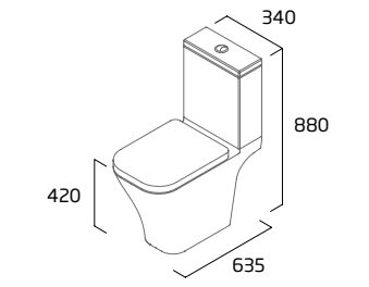
Comfort Height Standard Close Coupled WC
