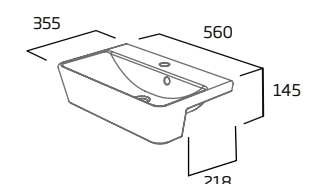
Slim Depth Semi-Countertop Basin 1 Tap Hole
