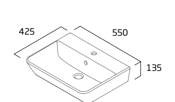
550 Basin
