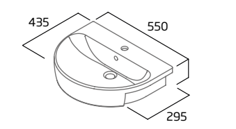
550mm Semi-Countertop Basin
