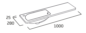
1000mm Isocast Basin - Left
