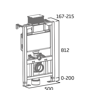
0.82m Wall Hung WC Frame
