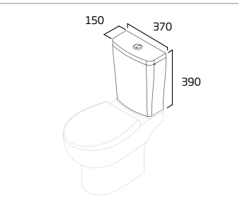
Standard WC Cistern
