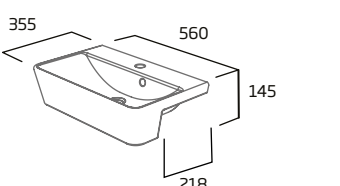
Slim Depth Semi-Countertop Basin
