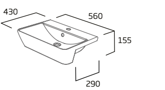
Semi-Countertop Basin
