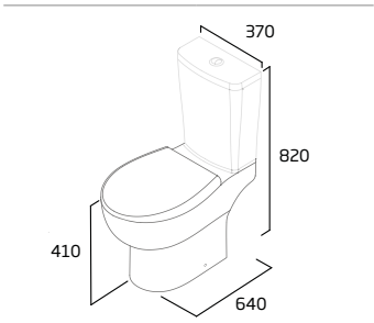
Standard Height Close Coupled WC
