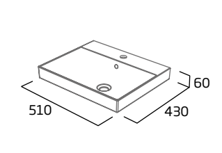
500mm Basin
