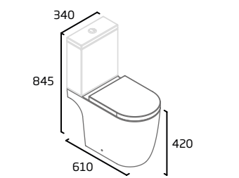
Standard Height Close Coupled WC
