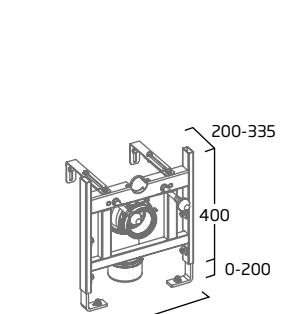
0.4m WC/Bidet Frame
