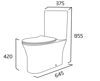
Standard Height Fully Enclosed Close Coupled WC
