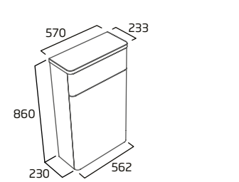
Back to Wall WC Unit
