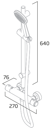
Joy Single Function Shower System
