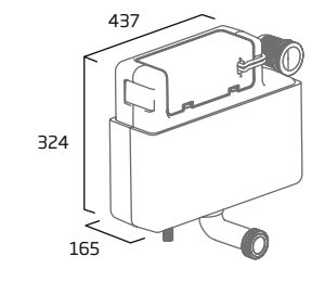
Comfort Height Cistern
