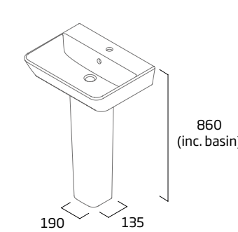
Pedestal
