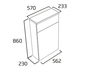
Back to Wall WC Unit
