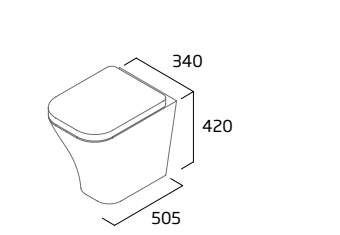
Back To Wall WC
