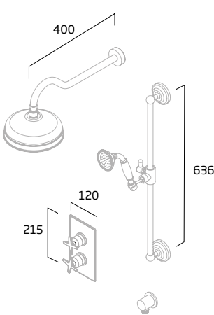
Ashton & Regatta Dual Function Shower System
