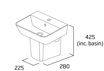
Semi Pedestal
