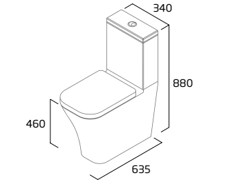
Comfort Height Fully Enclosed Close Coupled WC
