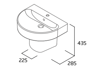
Semi Pedestal
