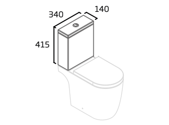
Standard WC Cistern with Contactless Flush
