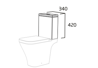
Standard WC Cistern (Fits Fully Enclosed and Open Back WC)
