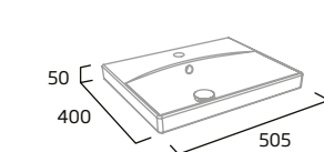
500mm Basin
