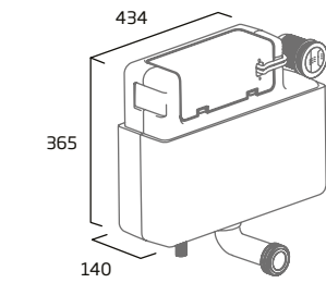
Concealed Dual Flush Cistern (Bottom Entry Inlet)
