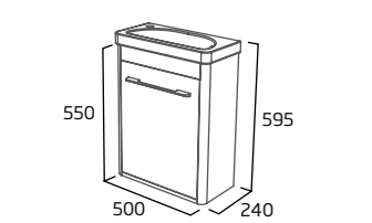
500mm Cloakroom Wall Mounted Wash Unit
