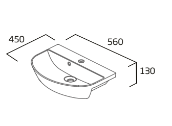
Standard Depth Semi-Countertop Basin
