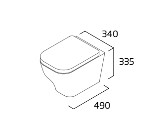
Wall Hung WC
