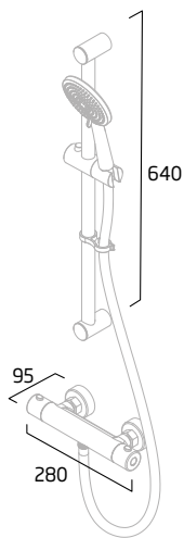
Joy Single Function Shower System
