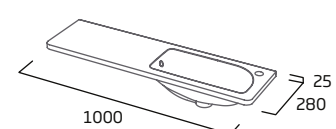
1000mm Isocast Basin - Right
