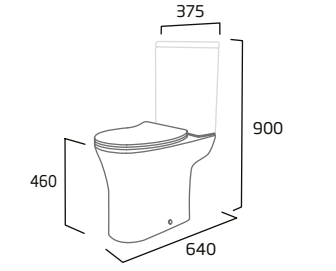
Comfort Height Close Coupled WC
