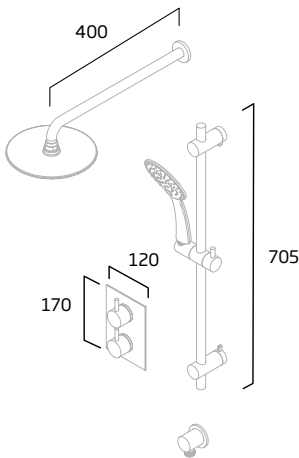
Fuse, Joy, Crew & Prefix Dual Function Shower System
