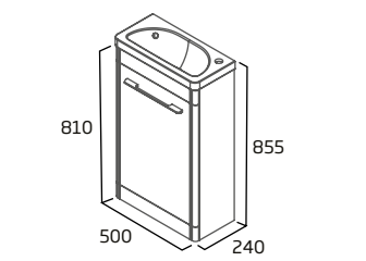
500mm Cloakroom Wash Unit
