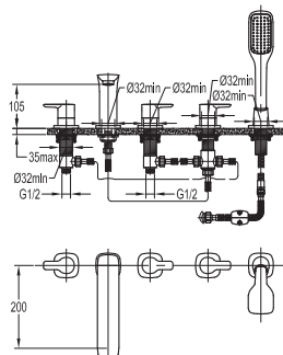
UR5HBSM 5-hole bath and shower mixer - 60mm x 60mm baseplates - Separate diverter control - Includes shower set with 1.8m pull out hose
