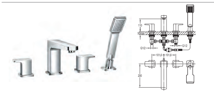
DE4HBSM 4-hole bath and shower mixer - 60mm x 60mm baseplates - Includes shower set with 1.8m pull out hose - Diverter behind the spout
