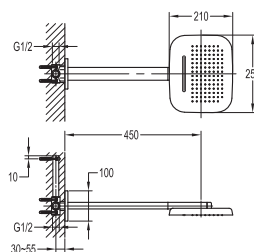
KI017 £477 Dual function rainshower with waterfall
