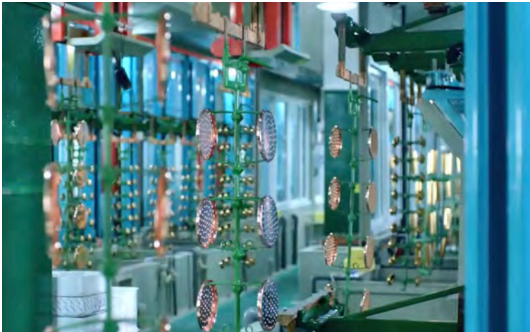
Automatic plating line - Our fully-automated plating line ensures a durable, accurate and mirror like finish everytime.
