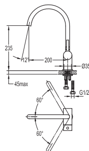
LVSLKITCH Single lever kitchen mixer - Swivel spout
