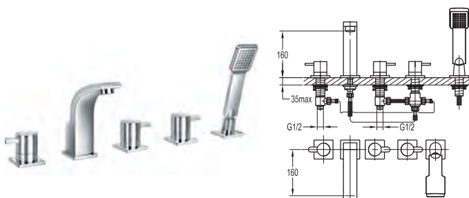
ES5HBSM 5-hole bath and shower mixer - 65mm x 65mm baseplates - Separate diverter control - Includes shower set with 1.8m pull out hose
