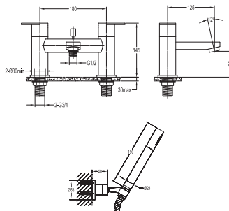
SMBSM Deck mounted bath and shower mixer - Includes shower kit with 1.5m hose
