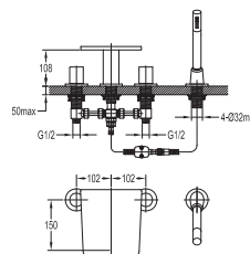
AN4HBSM 4-hole bath and shower mixer - Chrome
