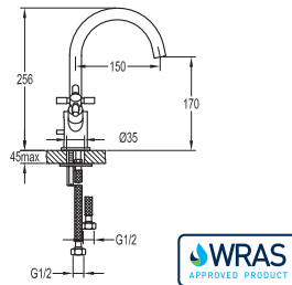
XLBAS 2-handle basin mixer - Includes clicker waste
