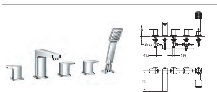
DE5HBSM 5-hole bath and shower mixer - 60mm x 60mm baseplates - Includes shower set with 1.8m pull out hose - Separate diverter control
