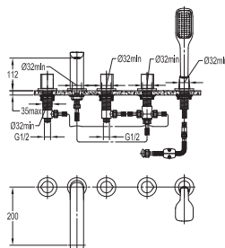
AL5HBSM 5-hole bath and shower mixer
