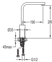
STKITCH Single lever kitchen mixer - Swivel spout
