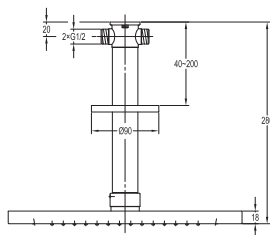
KI014 £590 Dual function rainshower with rainstream
