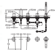
AN5HBSMGL 5-hole bath and shower mixer - Glass
